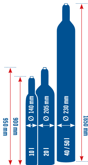
1 Gas cylinder
